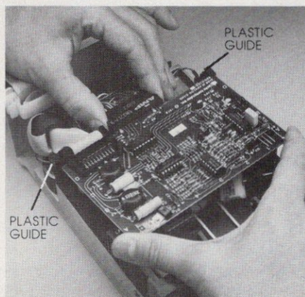
Figures 2 and 3: Removing the analog board: Unplug the read/write-head connector, unscrew the front retaining screws, and slide the board forward until it clears the plastic guides in the back.
