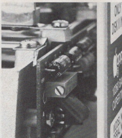
Figure 7: The disk-drive speed-adjustment screw is located inside the disk drive on the right side, in the rear. Using a speed-diagnostic program to display the speed of your drive, adjust the screw until the speed of the drive is within tolerance.
