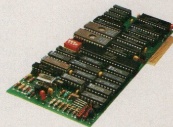
UltraTerm 128 × 32 display
